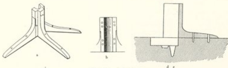
Fig. 278. — Mast-shoe.
