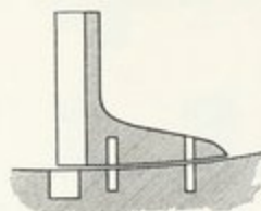
Fig. 70. — Mast-shoe, side view. Fig. 71. — Mast-shoe view of bottom. Fig. 72. — Mast-shoe, section.
