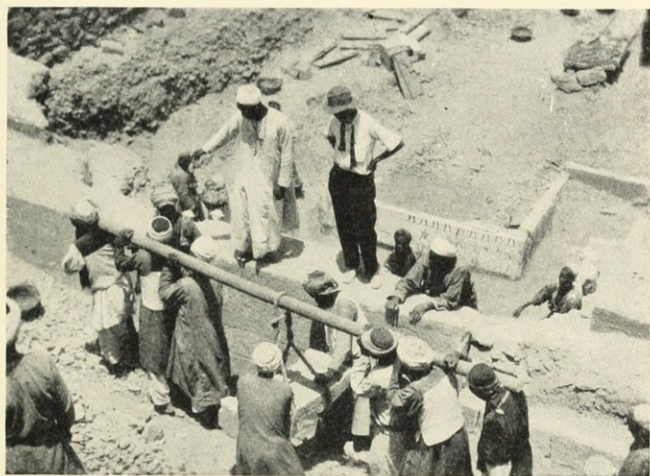
FIG. 23. METHOD OF CARRYING BLOCKS
