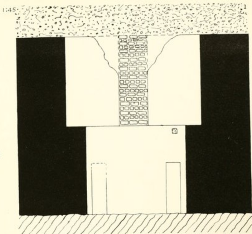
EAST TO WEST SECTION OF CENTRAL CHAMBER.
