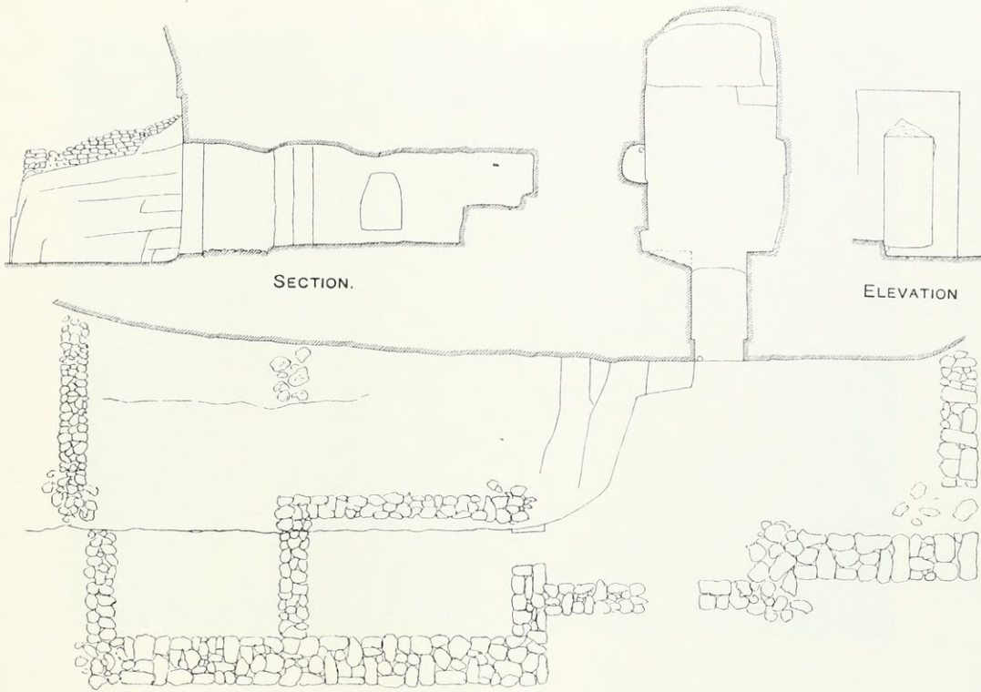
TOMB 6B. PLAN.
