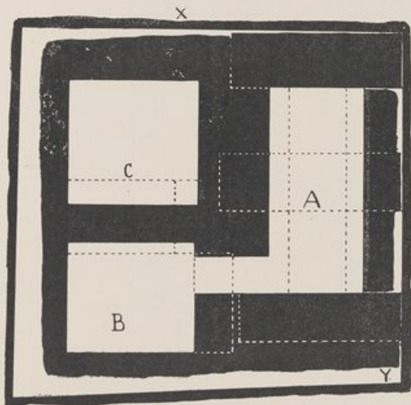
Tomb G. 64, ground plan, and enlarged plan of chambers showing vaulting. See p. 33
