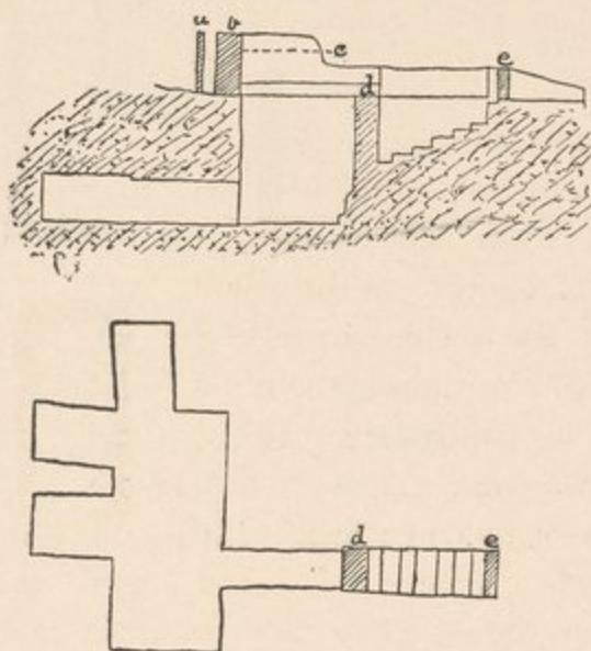
Section and ground-plan of K 37. Scale, 1 : 200.
