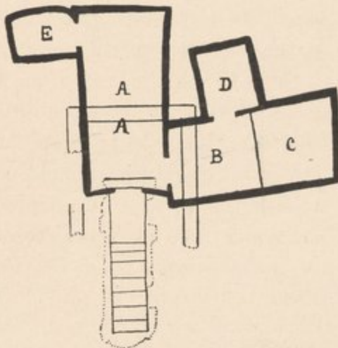
Superstructure and substructure of K 12. Scale, 1 : 200.
