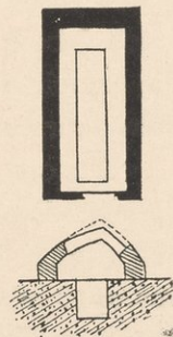
Ground-plan and section of K 19. Scale, 1 : 100.
