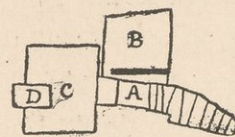
Section and ground-plan of K 27. Scale, 1 : 200.
