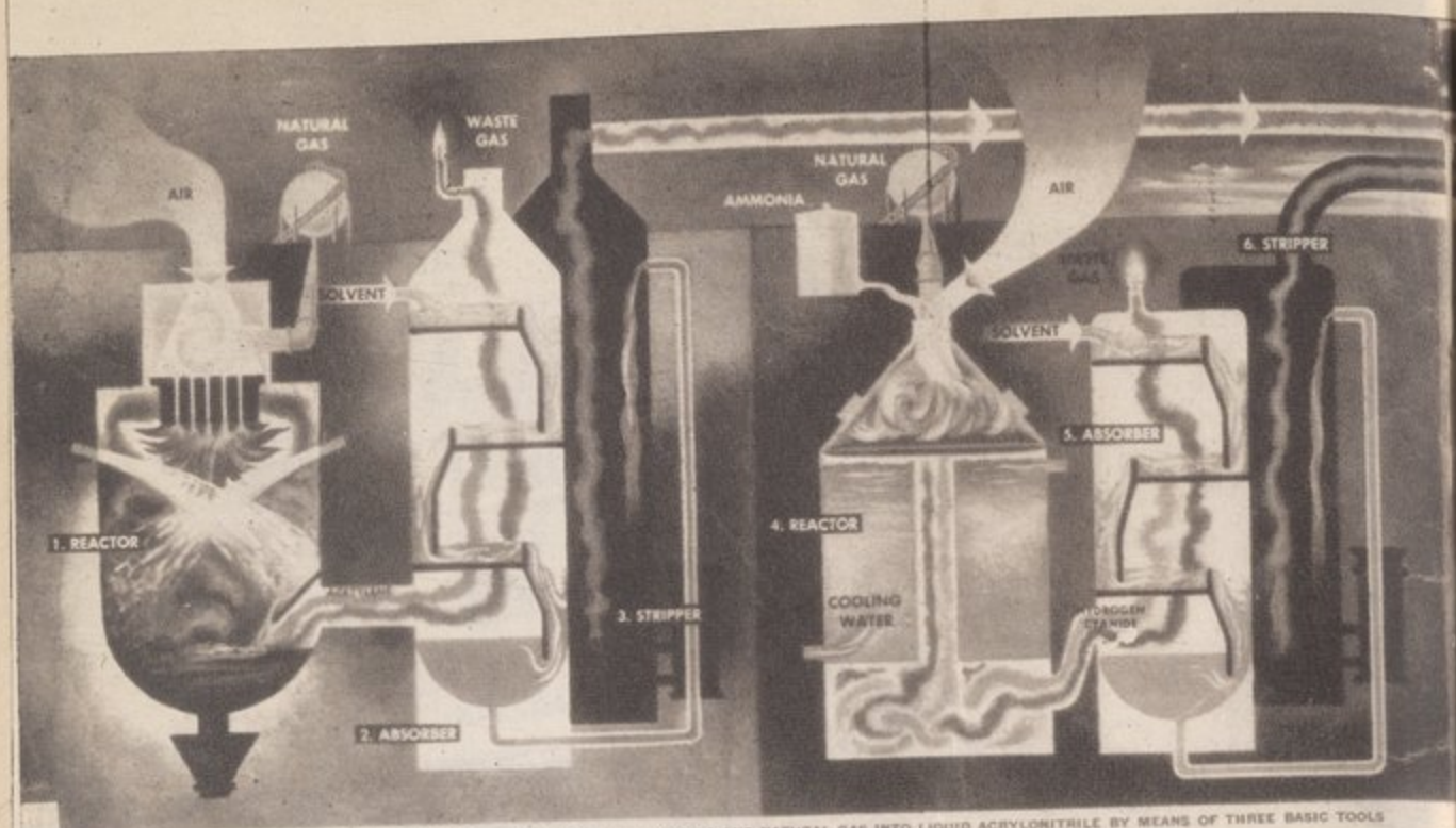
TEXAS CITY PROCESS, MAINLY CHEMICAL, TRANSFORMS AIR, AMMONIA AND NATURAL GAS INTO LIQUID ACRYLONITRILE BY MEANS OF THREE BASIC TOOLS
